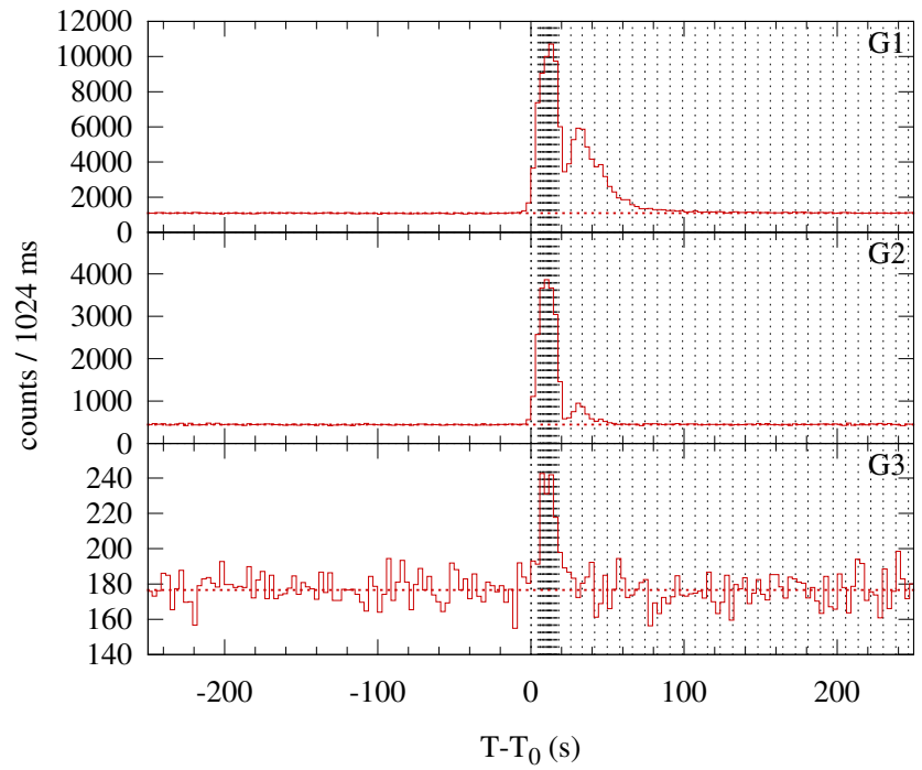
Konus-WIND S1 SOL1999-08-20T18:27 (M1.2) T_0 = 66450.302 s UT (18:27:30.302)
