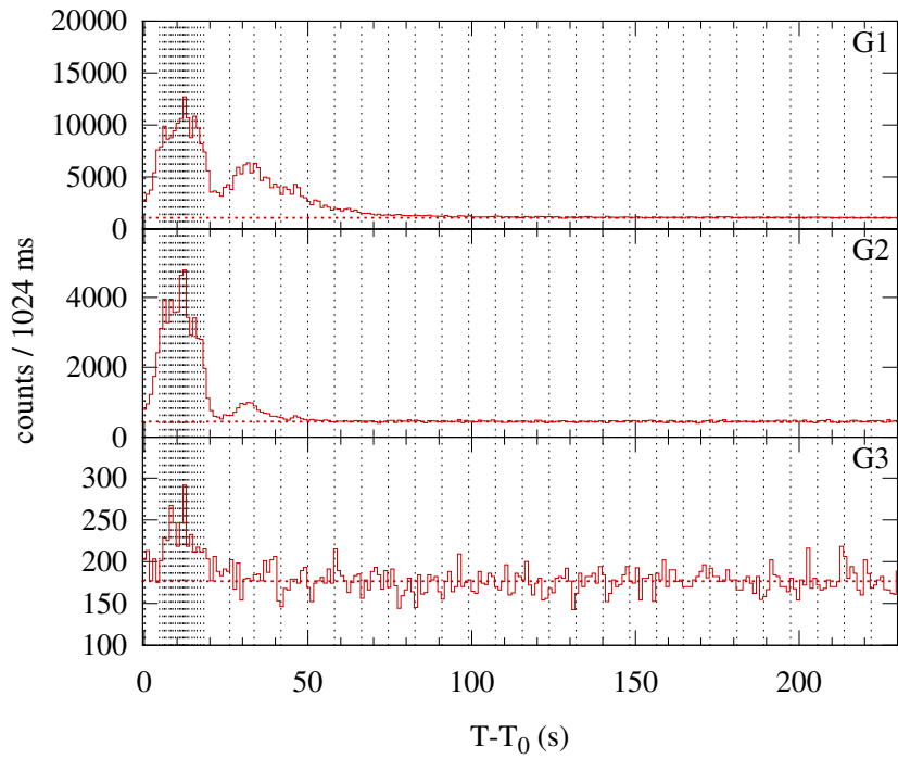
Konus-WIND S1 SOL1999-08-20T18:27 (M1.2) T_0 = 66450.302 s UT (18:27:30.302)
