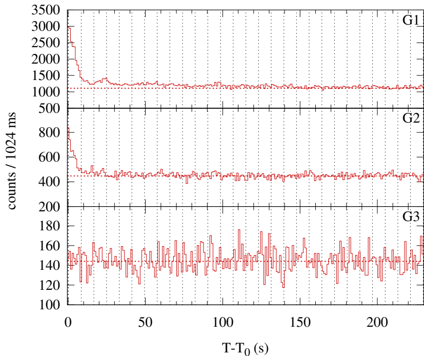
Konus-WIND S2 SOL1999-08-21T11:02 (C5.2) T 0 = 39761.910 s UT (11:02:41.910)
