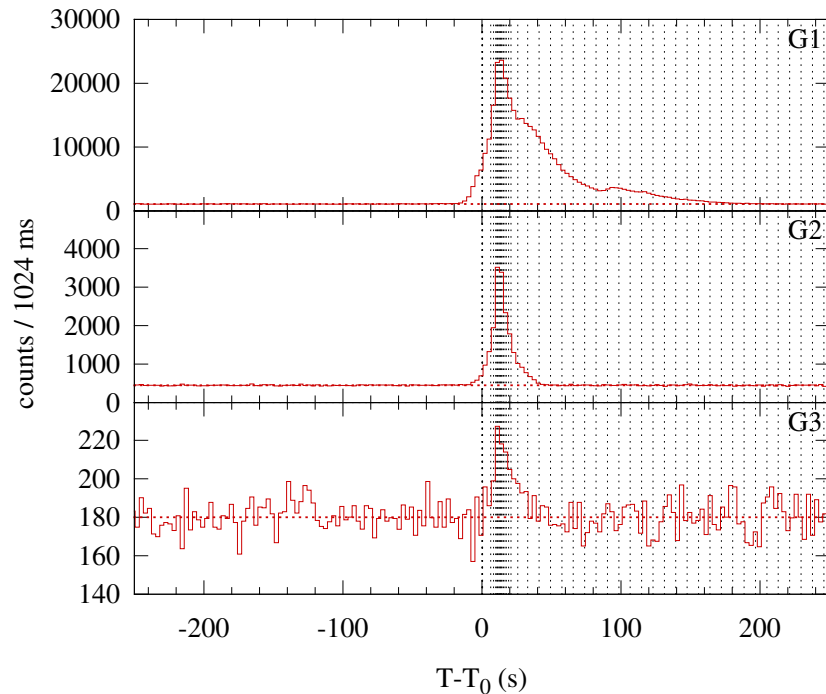
Konus-WIND S1 SOL1999-08-21T22:12 (M5.9) T_0 = 79974.694 s UT (22:12:54.694)
