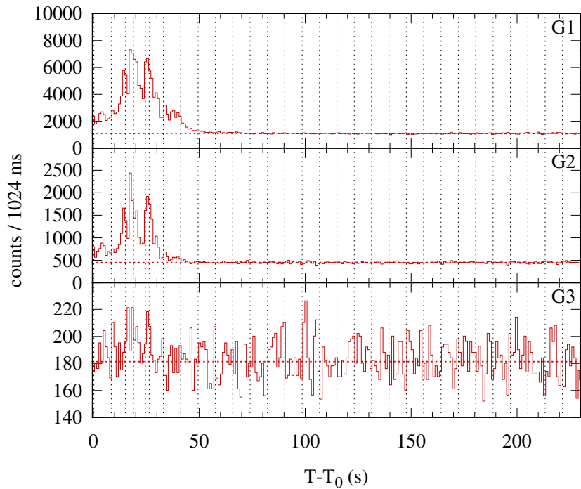
Konus-WIND S1 SOL1999-08-22T14:11 (C5.3) T 0 = 51060.264 s UT (14:11:00.264)
