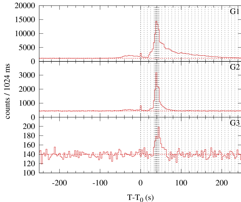
Konus-WIND S2 SOL1999-08-25T01:34 (M3.6) T_0 = 5692.634 s UT (01:34:52.634)
