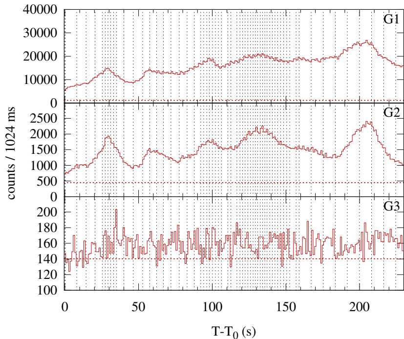
Konus-WIND S2 SOL1999-08-28T17:55 (X1.1) T_0 = 64550.744 s UT (17:55:50.744)
