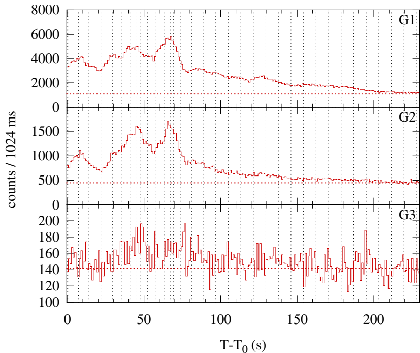
Konus-WIND S2 SOL1999-09-08T12:13 (M1.4) T_0 = 44035.527 s UT (12:13:55.527)
