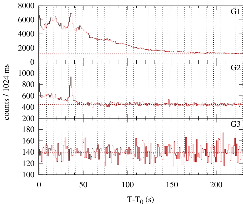
Konus-WIND S2 SOL1999-09-17T01:18 (M2.1) T_0 = 4699.213 s UT (01:18:19.213)
