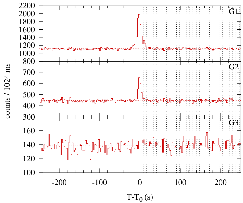
Konus-WIND S2 SOL1999-09-18T18:20 (C2.3) T_0 = 66011.679 s UT (18:20:11.679)
