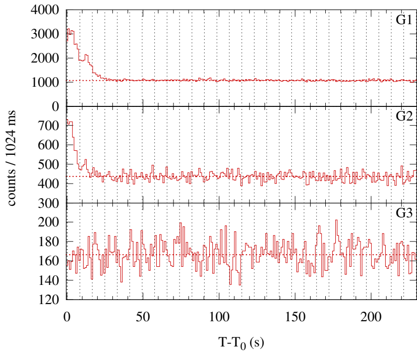
Konus-WIND S1 SOL1999-11-09T15:34 (C4.4) T_0 = 56083.106 s UT (15:34:43.106)
