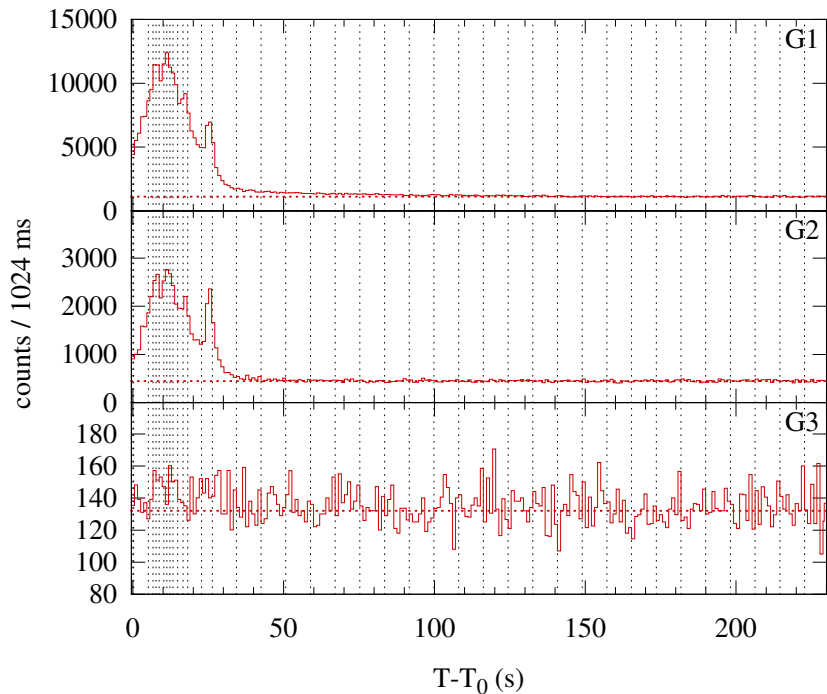
Konus-WIND S2 SOL1999-11-10T22:11 (M1.1) T_0 = 79910.91 s UT (22:11:50.91)
