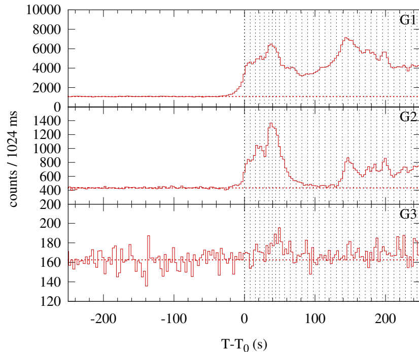
Konus-WIND S1 SOL1999-11-14T07:56 (M8.0) T 0 = 28615.332 s UT (07:56:55.332)
