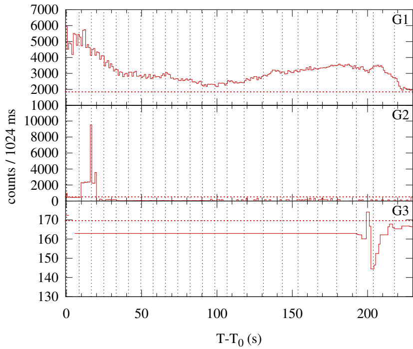
Konus-WIND S1 SOL1999-11-14T16:22 (M2.2) T_0 = 58925.840 s UT (16:22:05.840)
