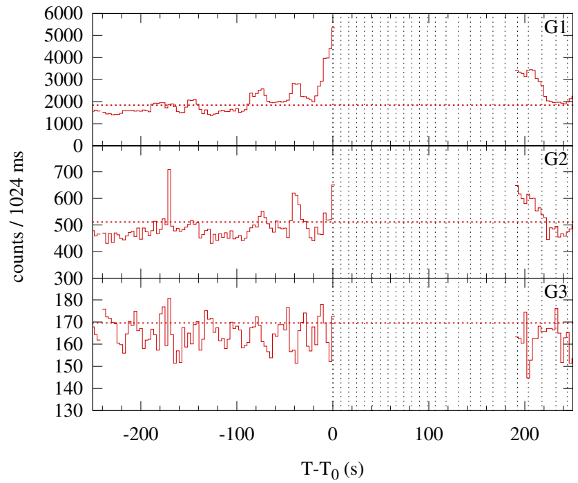
Konus-WIND S1 SOL1999-11-14T16:22 (M2.2) T_0 = 58925.840 s UT (16:22:05.840)
