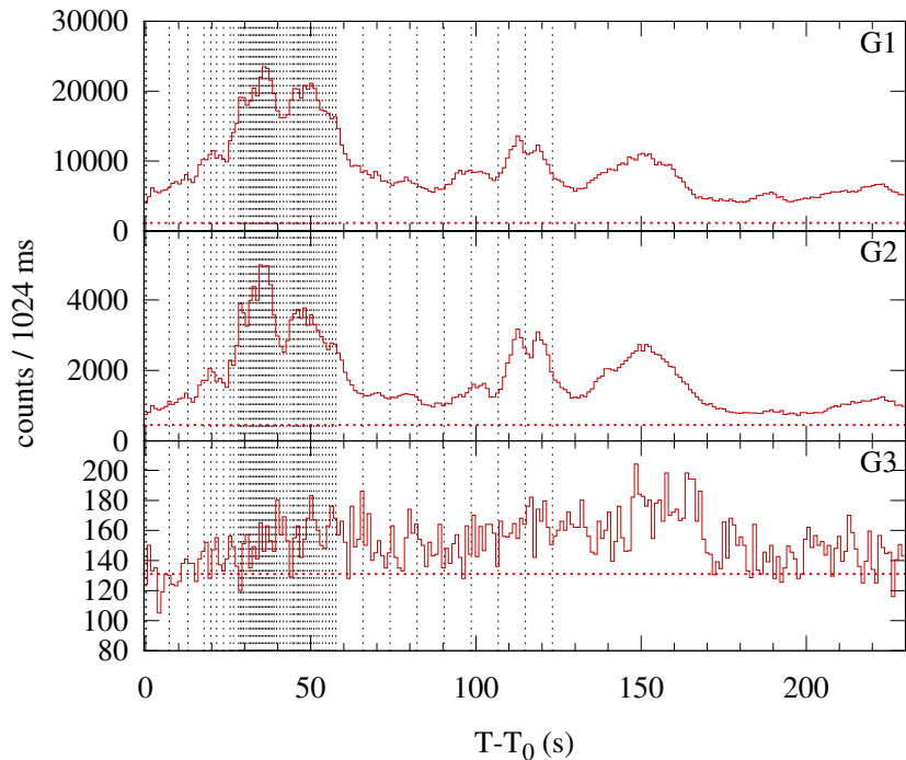
Konus-WIND S2 SOL1999-11-17T09:52 (M7.4) T_0 = 35523.586 s UT (09:52:03.586)
