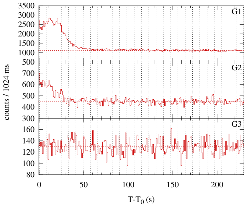
Konus-WIND S2 SOL1999-11-22T02:54 (C2.9) T 0 = 10479.287 s UT (02:54:39.287)
