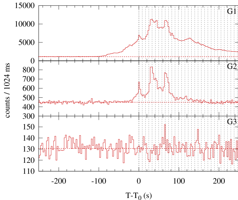
Konus-WIND S2 SOL1999-11-26T01:19 (M5.7) T 0 = 4768.241 s UT (01:19:28.241)
