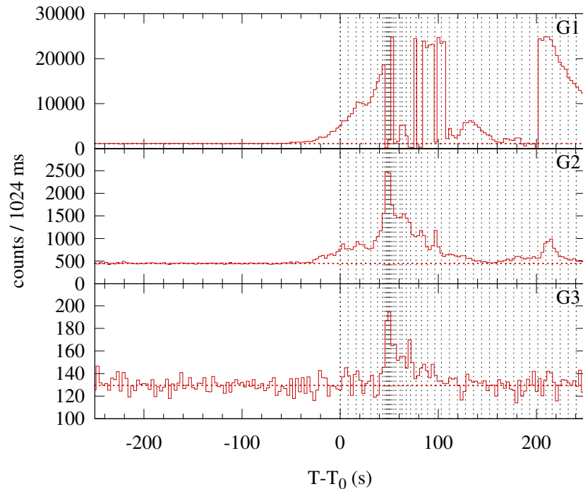
Konus-WIND S2 SOL1999-11-27T12:08 (X1.4) T_0 = 43735.804 s UT (12:08:55.804)
