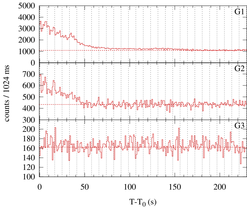
Konus-WIND S1 SOL1999-11-28T11:52 (C5.3) T 0 = 42759.855 s UT (11:52:39.855)
