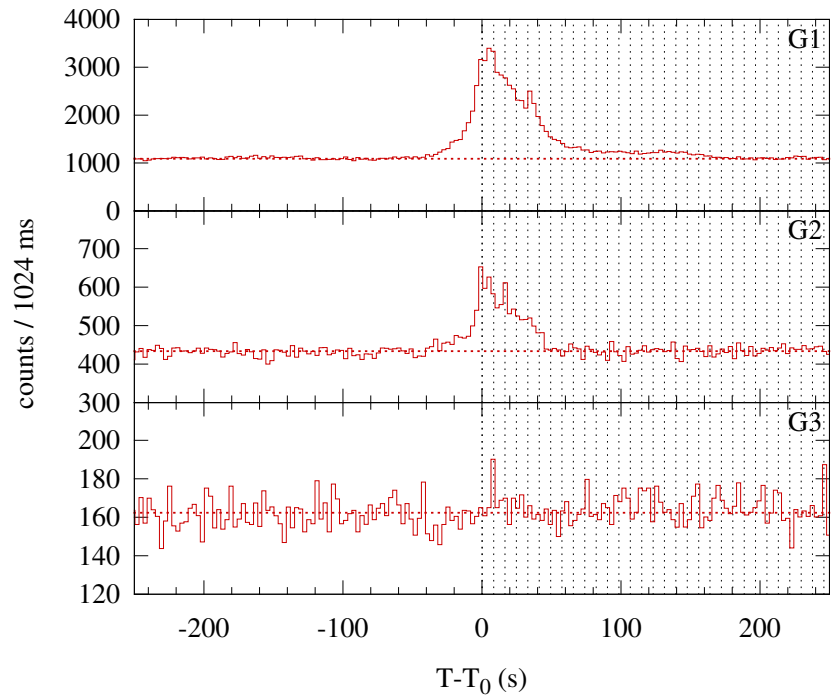
Konus-WIND S1 SOL1999-11-28T11:52 (C5.3) T 0 = 42759.855 s UT (11:52:39.855)
