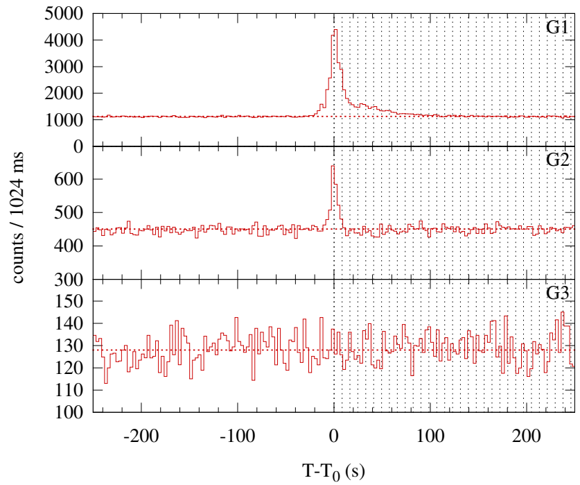
Konus-WIND S2 SOL1999-12-17T09:33 (C4.9) T 0 = 34418.750 s UT (09:33:38.750)
