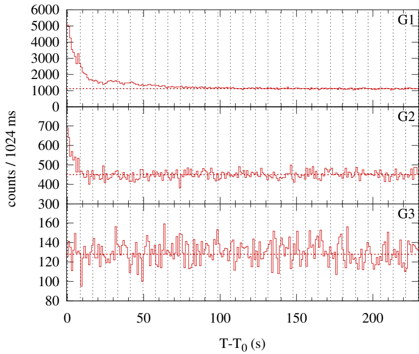
Konus-WIND S2 SOL1999-12-17T09:33 (C4.9) T 0 = 34418.750 s UT (09:33:38.750)
