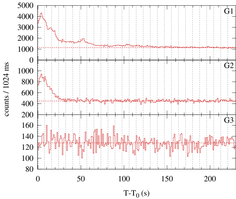
Konus-WIND S2 SOL1999-12-17T21:38 (M1.0) T 0 = 77921.553 s UT (21:38:41.553)
