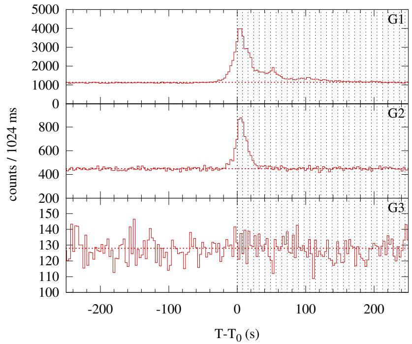
Konus-WIND S2 SOL1999-12-17T21:38 (M1.0) T 0 = 77921.553 s UT (21:38:41.553)
