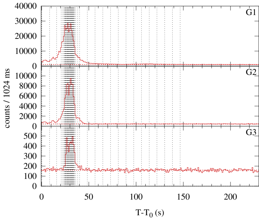
Konus-WIND S1 SOL1999-12-18T19:11 (M1.5) T_0 = 69087.126 s UT (19:11:27.126)
