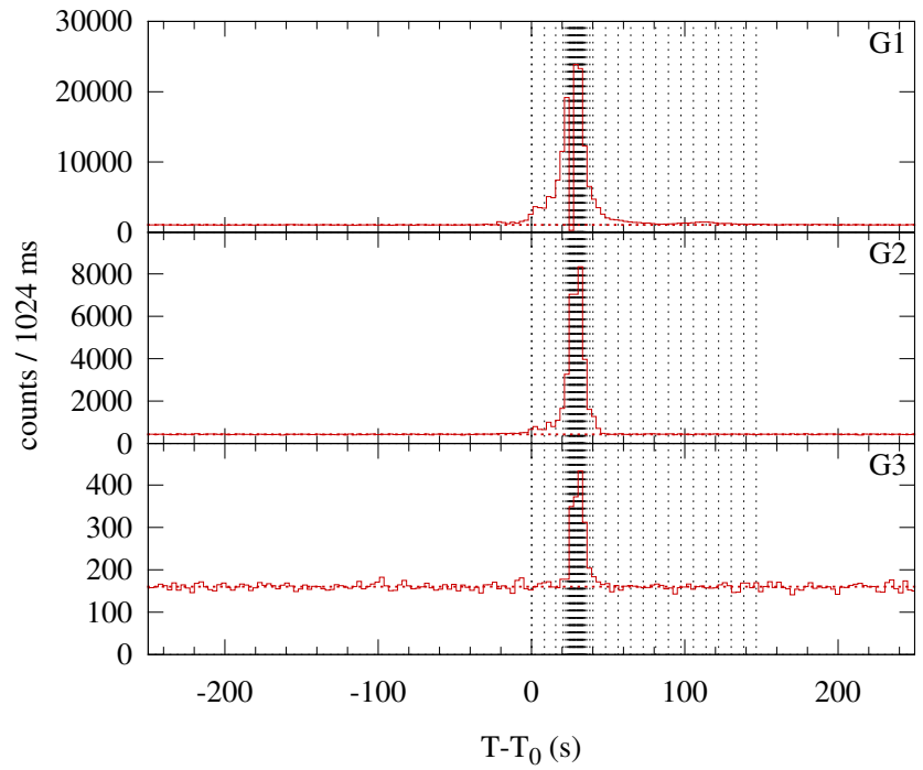
Konus-WIND S1 SOL1999-12-18T19:11 (M1.5) T_0 = 69087.126 s UT (19:11:27.126)
