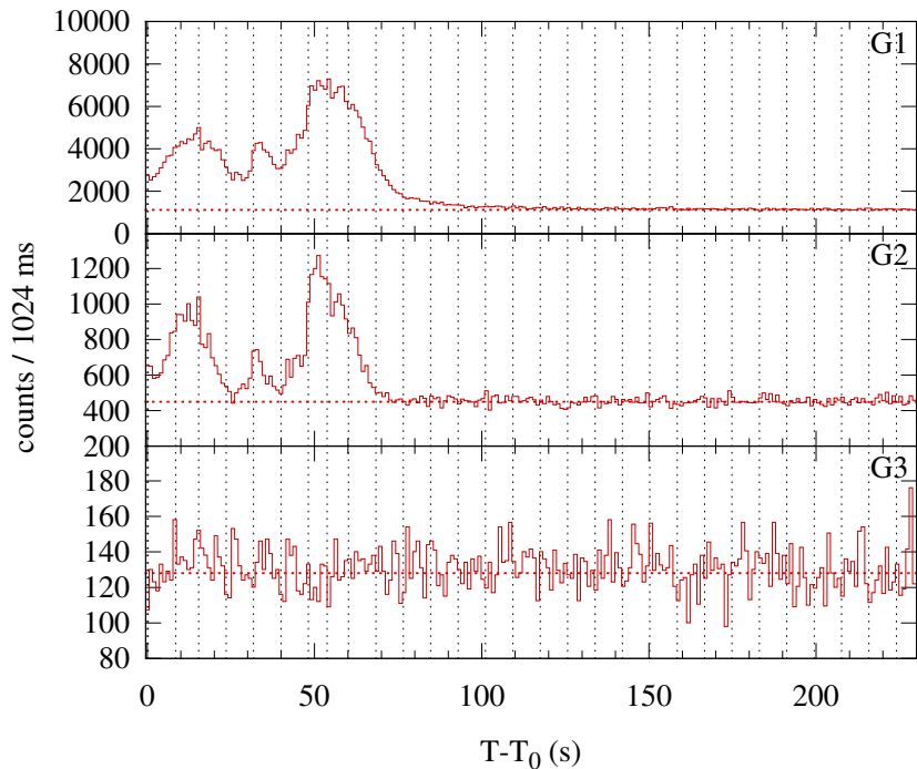
Konus-WIND S2 SOL1999-12-22T10:53 (C6.3) T_0 = 39200.862 s UT (10:53:20.862)
