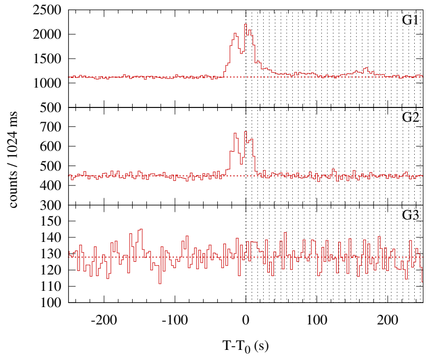
Konus-WIND S2 SOL1999-12-22T18:55 (M5.3) T 0 = 68108.709 s UT (18:55:08.709)
