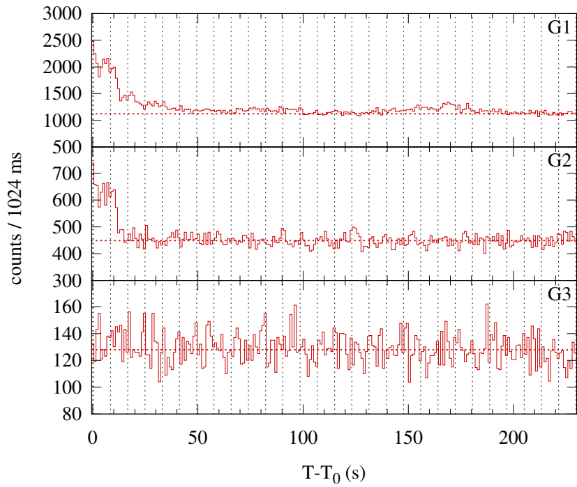
Konus-WIND S2 SOL1999-12-22T18:55 (M5.3) T 0 = 68108.709 s UT (18:55:08.709)
