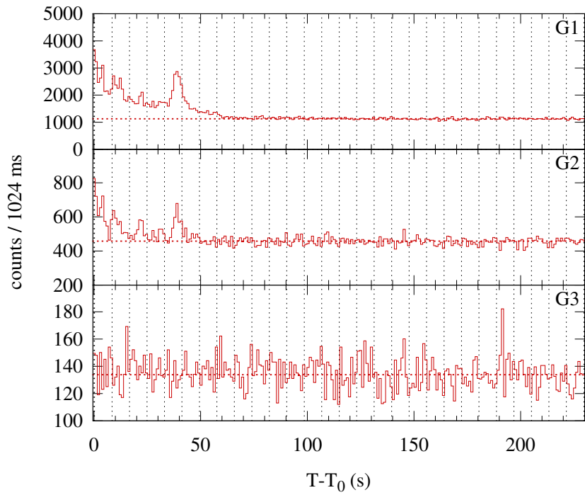
Konus-WIND S2 SOL1999-12-23T10:07 (C2.9) T_0 = 36449.303 s UT (10:07:29.303)
