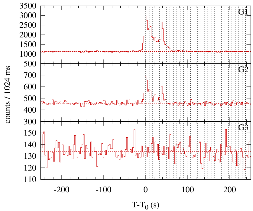
Konus-WIND S2 SOL1999-12-23T10:07 (C2.9) T_0 = 36449.303 s UT (10:07:29.303)
