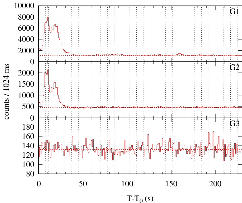
Konus-WIND S2 SOL1999-12-23T19:33 (C3.4) T_0 = 70395.920 s UT (19:33:15.920)
