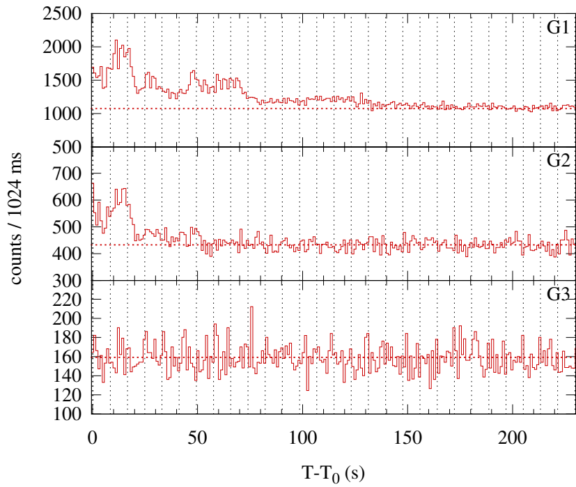
Konus-WIND S1 SOL1999-12-25T11:26 (C6.2) T 0 = 41188.256 s UT (11:26:28.256)
