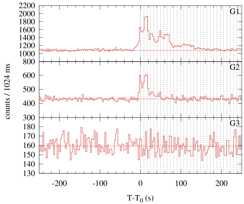
Konus-WIND S1 SOL1999-12-25T11:26 (C6.2) T 0 = 41188.256 s UT (11:26:28.256)
