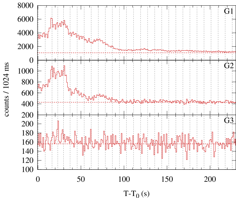
Konus-WIND S1 SOL1999-12-27T01:49 (M1.0) T 0 = 6585.858 s UT (01:49:45.858)
