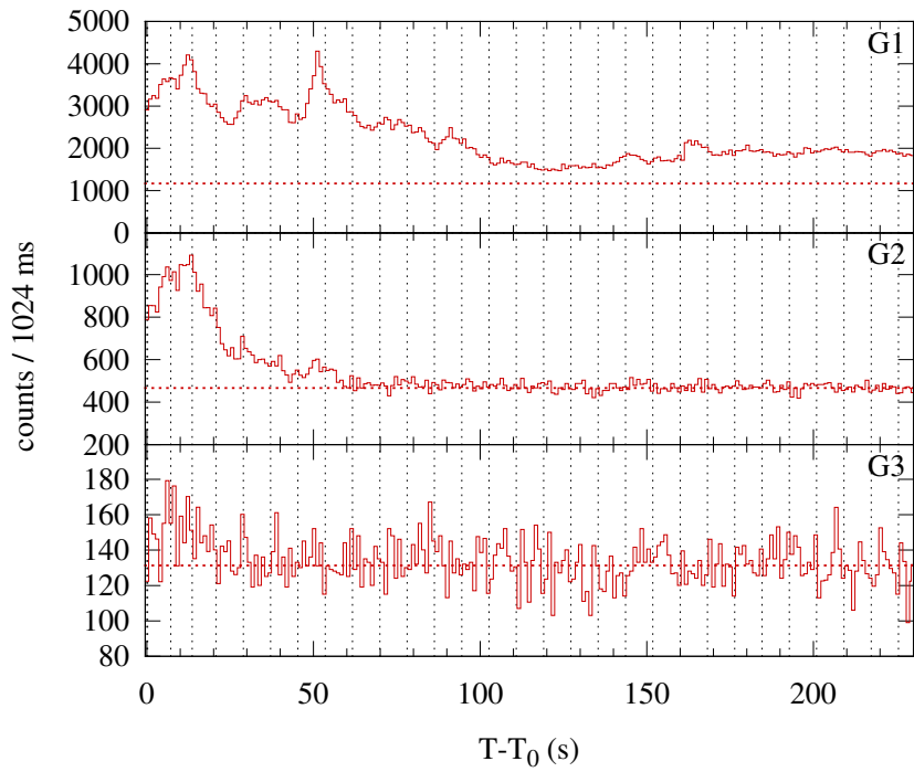
Konus-WIND S2 SOL1999-12-27T12:00 (M2.0) T_0 = 43203.456 s UT (12:00:03.456)
