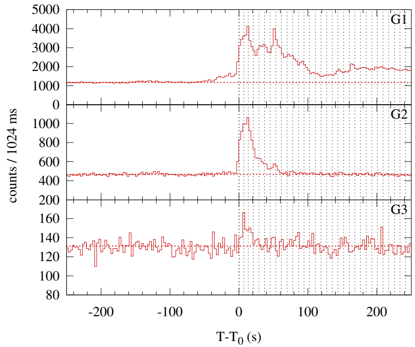
Konus-WIND S2 SOL1999-12-27T12:00 (M2.0) T_0 = 43203.456 s UT (12:00:03.456)
