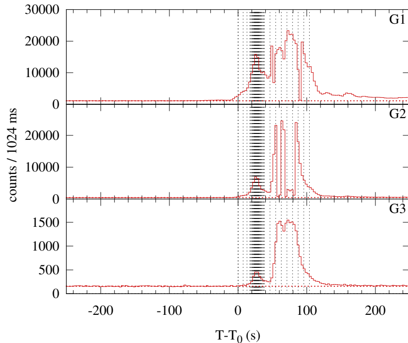
Konus-WIND S1 SOL1999-12-28T00:42 (M4.5) T 0 = 2572.87 s UT (00:42:52.87)
