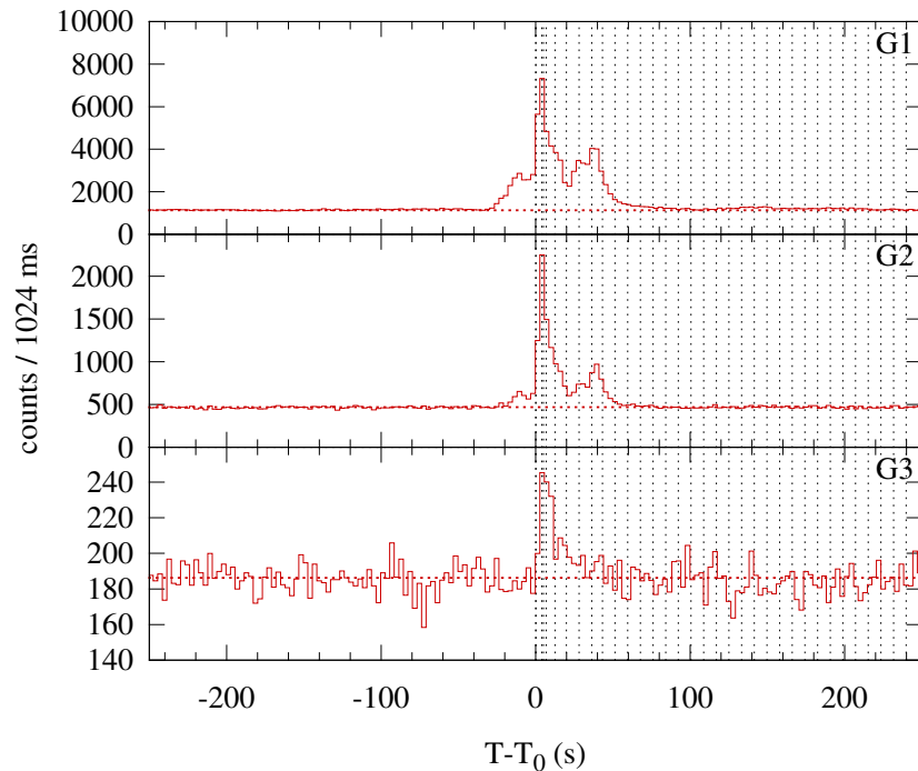
Konus-WIND S1 SOL1999-12-29T09:25 (C8.8) T_0 = 33921.917 s UT (09:25:21.917)
