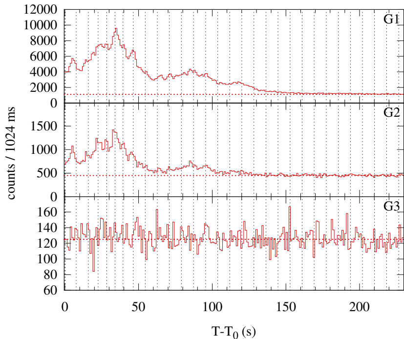
Konus-WIND S2 SOL2000-01-22T17:58 (M1.0) T 0 = 64724.472 s UT (17:58:44.472)
