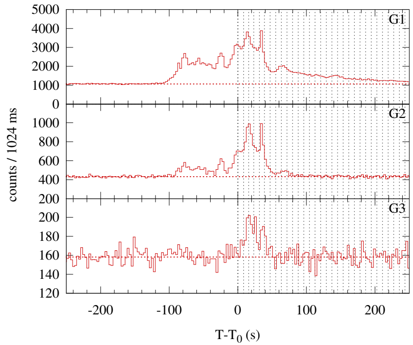
Konus-WIND S1 SOL2000-02-20T22:05 (M2.4) T 0 = 79521.790 s UT (22:05:21.790)
