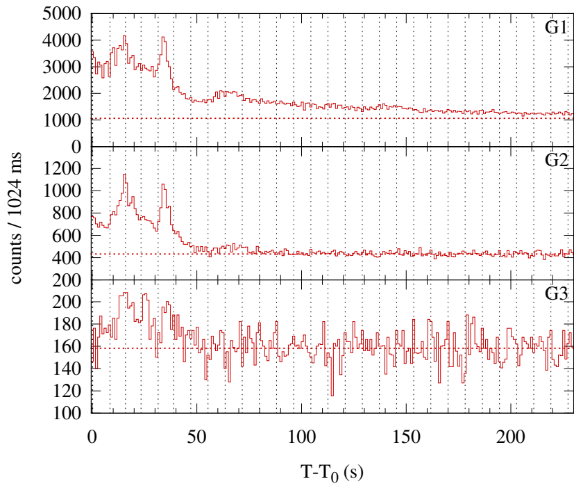
Konus-WIND S1 SOL2000-02-20T22:05 (M2.4) T 0 = 79521.790 s UT (22:05:21.790)
