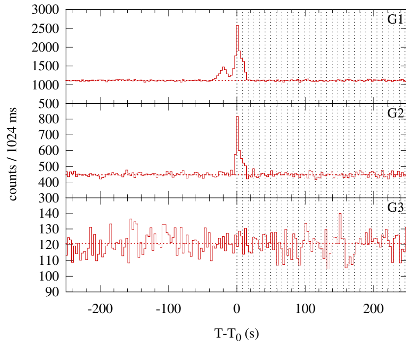
Konus-WIND S2 SOL2000-03-01T11:47 (C1.3) T 0 = 42468.980 s UT (11:47:48.980)
