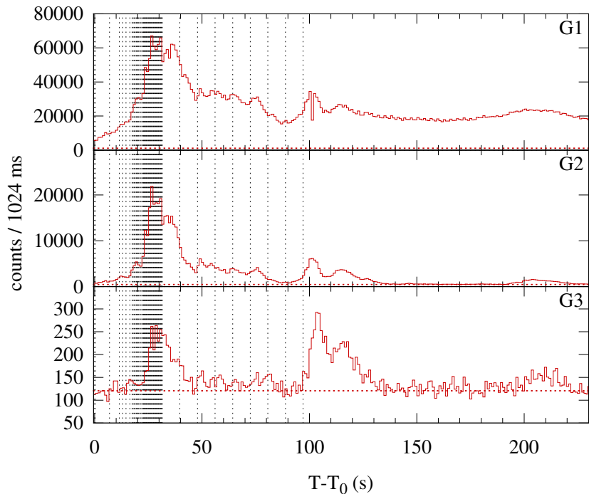
Konus-WIND S2 SOL2000-03-02T08:23 (X1.1) T_0 = 30236.631 s UT (08:23:56.631)
