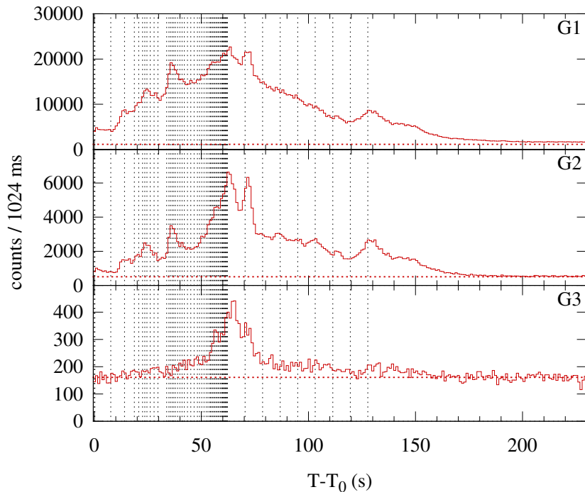
Konus-WIND S2 SOL2000-03-03T02:11 (M3.8) T_0 = 7886.527 s UT (02:11:26.527)
