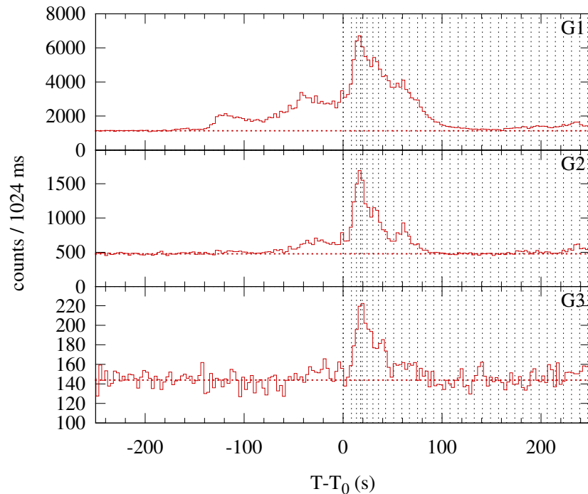
Konus-WIND S2 SOL2000-03-03T10:45 (M4.0) T 0 = 38714.481 s UT (10:45:14.481)
