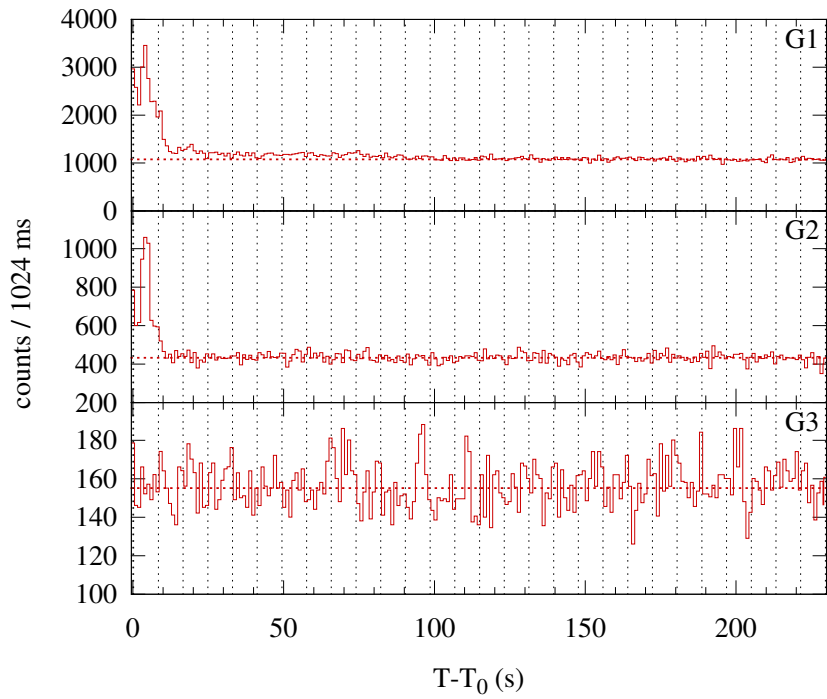
Konus-WIND S1 SOL2000-03-07T15:11 (C5.1) T 0 = 54685.866 s UT (15:11:25.866)
