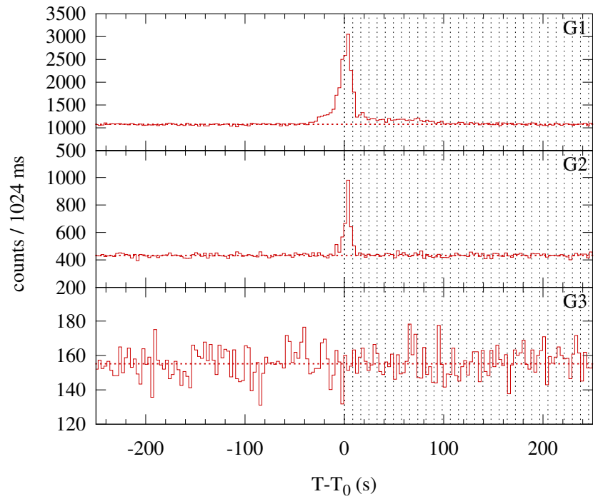
Konus-WIND S1 SOL2000-03-07T15:11 (C5.1) T 0 = 54685.866 s UT (15:11:25.866)
