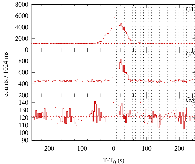
Konus-WIND S2 SOL2000-03-12T09:03 (C5.8) T_0 = 32604.557 s UT (09:03:24.557)
