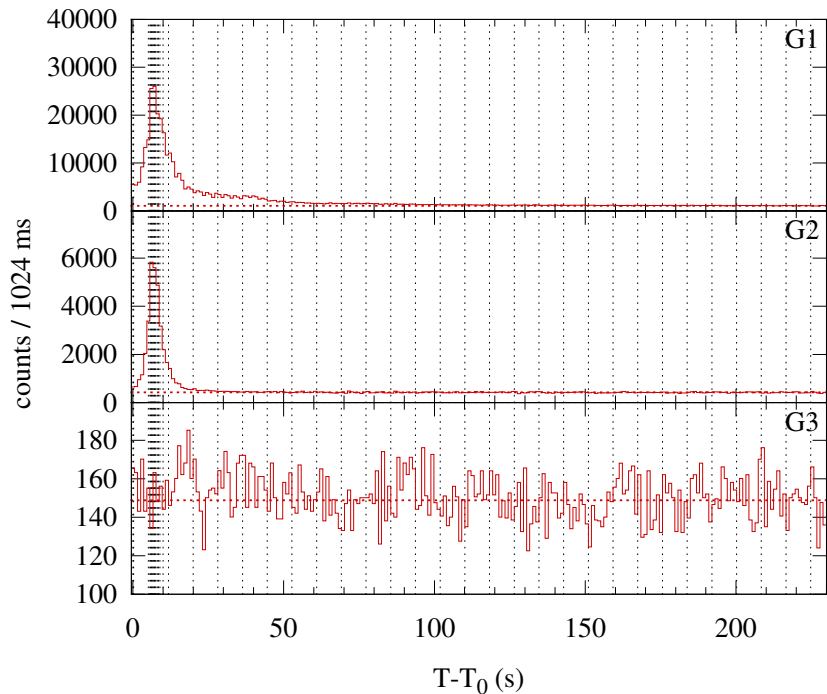
Konus-WIND S1 SOL2000-03-13T05:03 (C6.8) T 0 = 18189.791 s UT (05:03:09.791)
