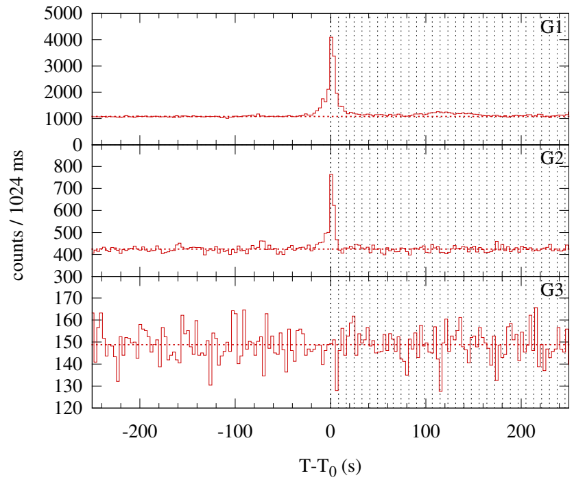
Konus-WIND S1 SOL2000-03-15T05:40 (C4.0) T_0 = 20451.425 s UT (05:40:51.425)
