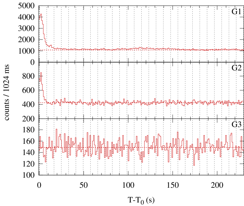
Konus-WIND S1 SOL2000-03-15T05:40 (C4.0) T_0 = 20451.425 s UT (05:40:51.425)
