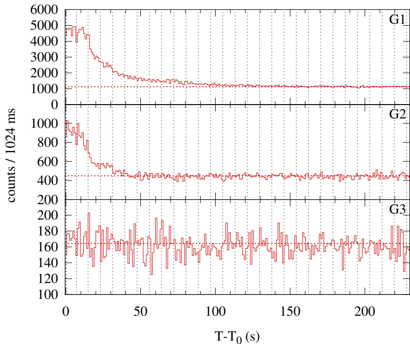
Konus-WIND S1 SOL2000-03-23T00:28 (M1.3) T_0 = 1698.467 s UT (00:28:18.467)
