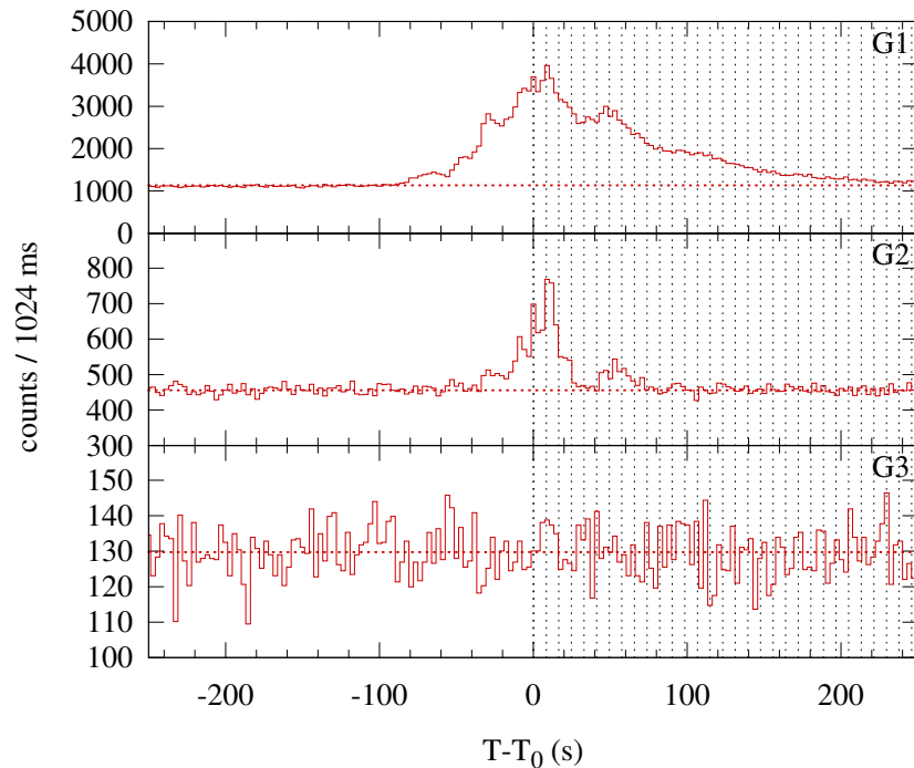
Konus-WIND S2 SOL2000-03-24T11:27 (M2.8) T_0 = 41279.472 s UT (11:27:59.472)
