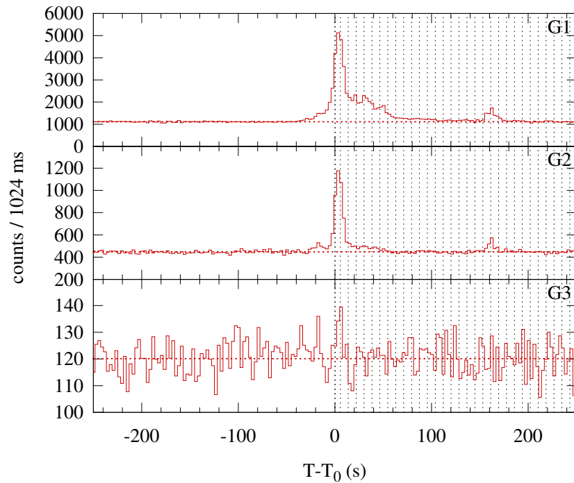
Konus-WIND S2 SOL2000-03-27T13:58 (C8.4) T_0 = 50339.323 s UT (13:58:59.323)
