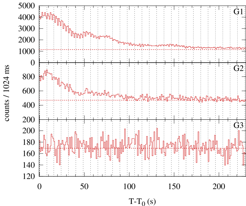
Konus-WIND S1 SOL2000-04-06T02:22 (M1.8) T_0 = 8548.433 s UT (02:22:28.433)
