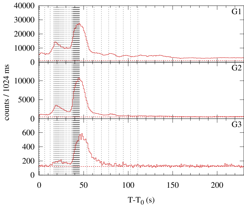
Konus-WIND S2 SOL2000-05-02T14:45 (M2.8) T 0 = 53141.440 s UT (14:45:41.440)
