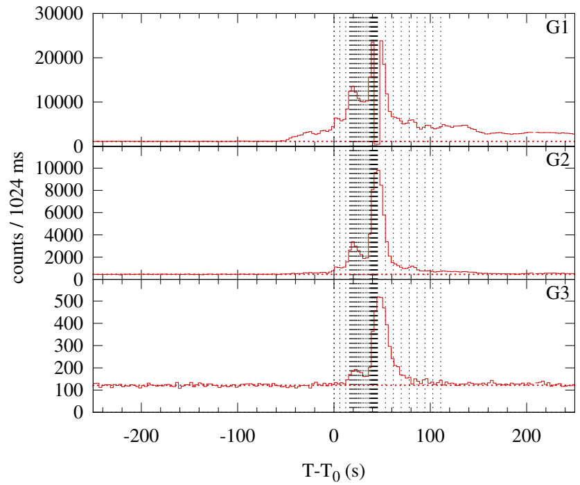
Konus-WIND S2 SOL2000-05-02T14:45 (M2.8) T 0 = 53141.440 s UT (14:45:41.440)
