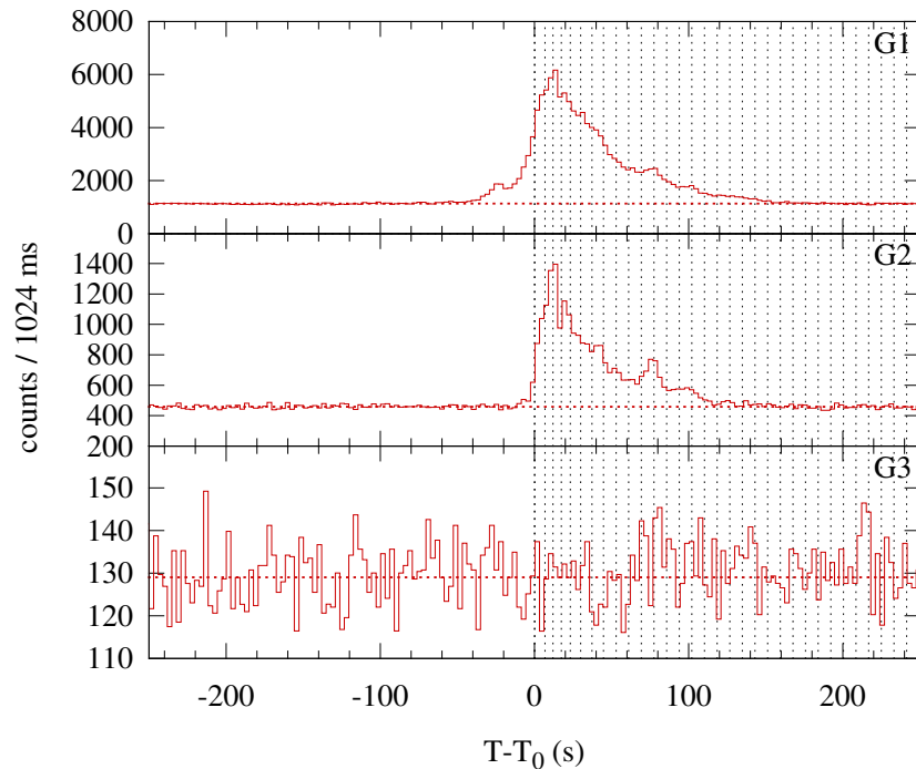
Konus-WIND S2 SOL2000-05-14T09:16 (C7.5) T 0 = 33418.422 s UT (09:16:58.422)
