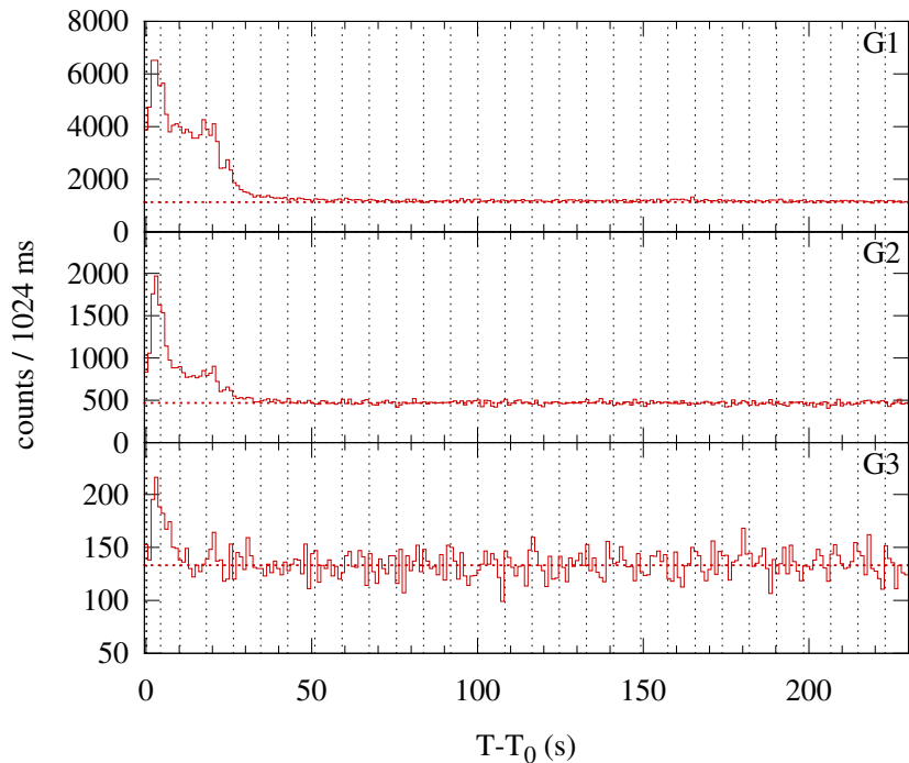
Konus-WIND S2 SOL2000-05-15T10:48 (M1.2) T_0 = 38914.516 s UT (10:48:34.516)
