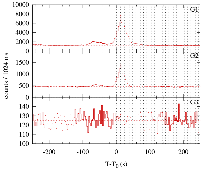
Konus-WIND S2 SOL2000-05-21T10:21 (C8.2) T_0 = 37273.155 s UT (10:21:13.155)
