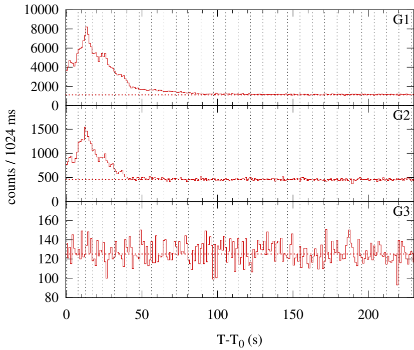
Konus-WIND S2 SOL2000-05-21T10:21 (C8.2) T_0 = 37273.155 s UT (10:21:13.155)
