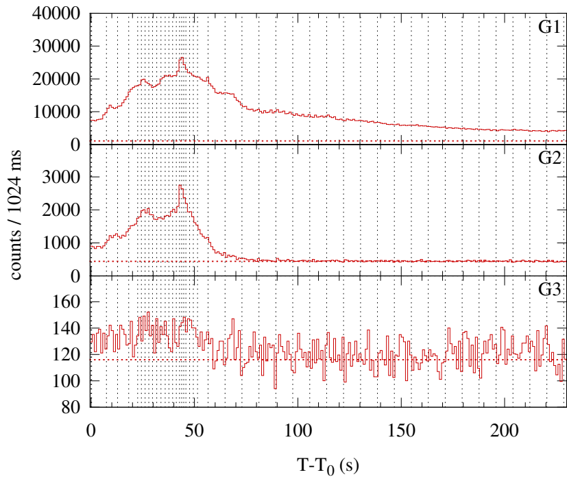
Konus-WIND S2 SOL2000-06-03T19:18 (M6.1) T_0 = 69502.400 s UT (19:18:22.400)
