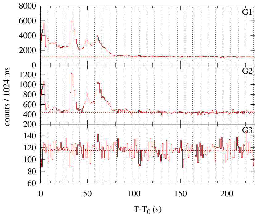
Konus-WIND S2 SOL2000-06-15T15:12 (C6.6) T 0 = 54774.369 s UT (15:12:54.369)
